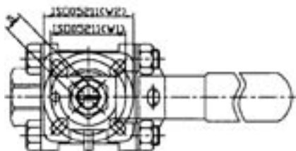
4" FULL PORT
